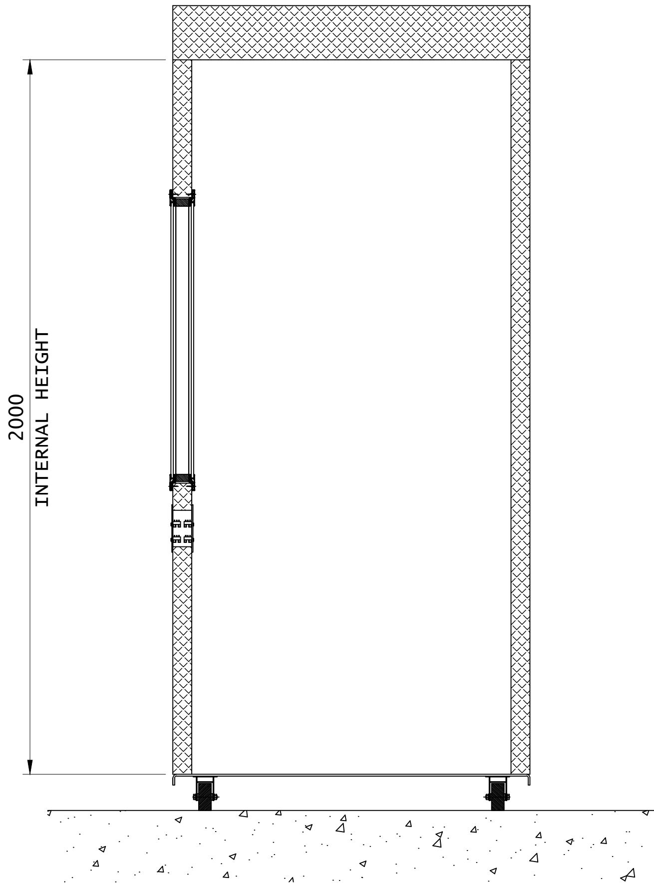
SECTION "A-A"
