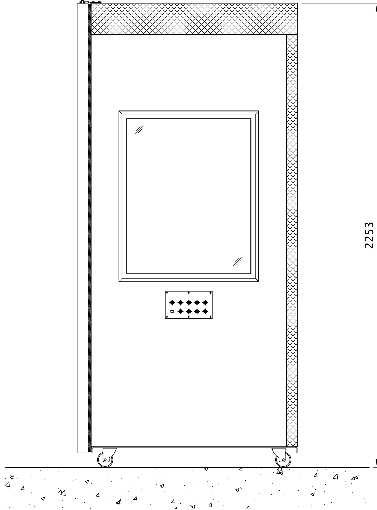
SECTION "B-B"
